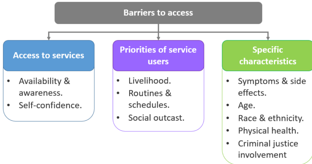
Figure 2: Theme map
