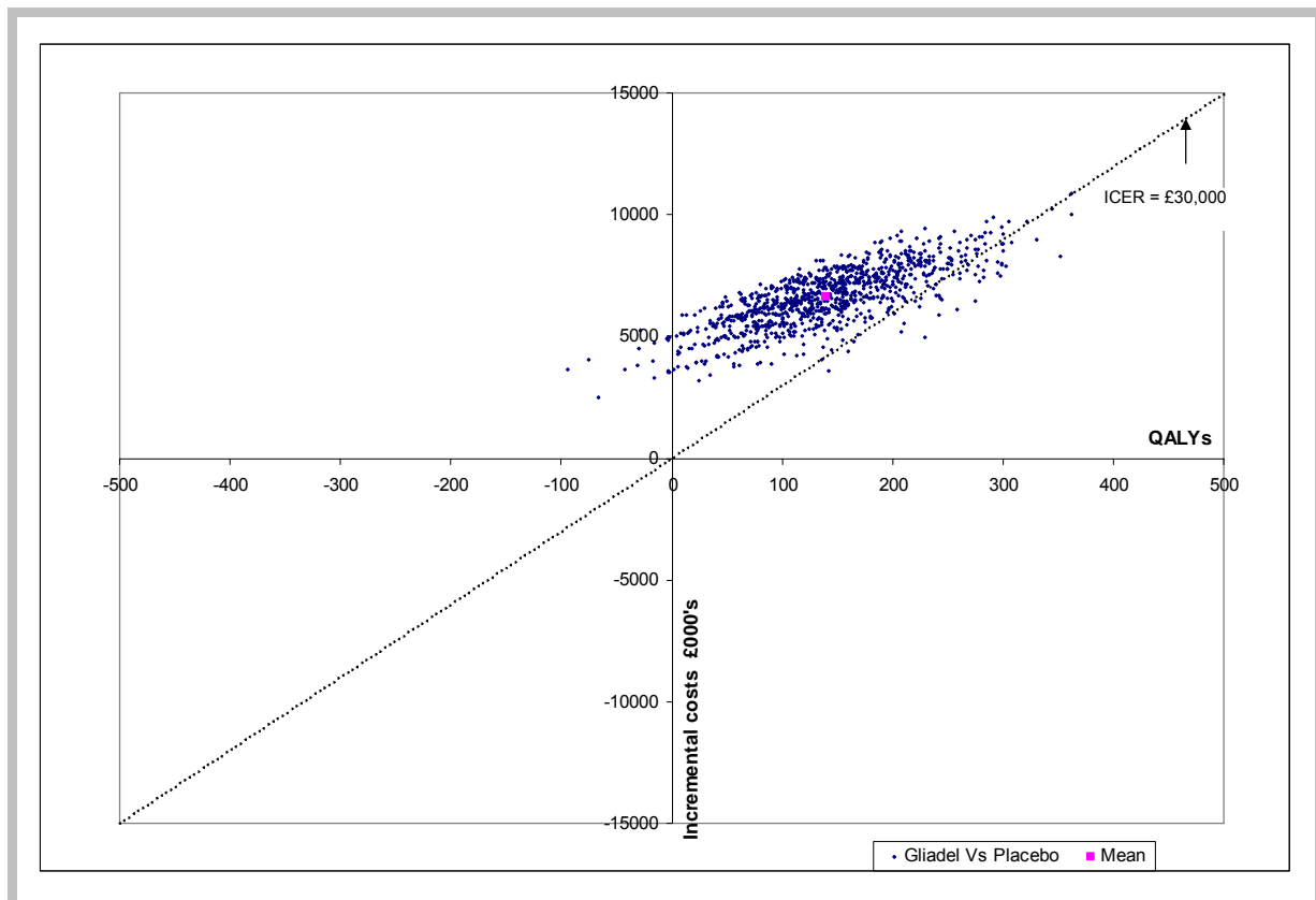
FIGURE 24 Simulation output (1000 trials) for cost-effectiveness of BCNU-W
