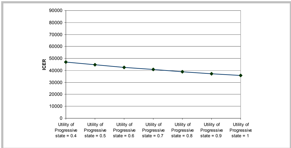
FIGURE 32 Threshold analysis for utility value in “progressive” disease state with TMZ
