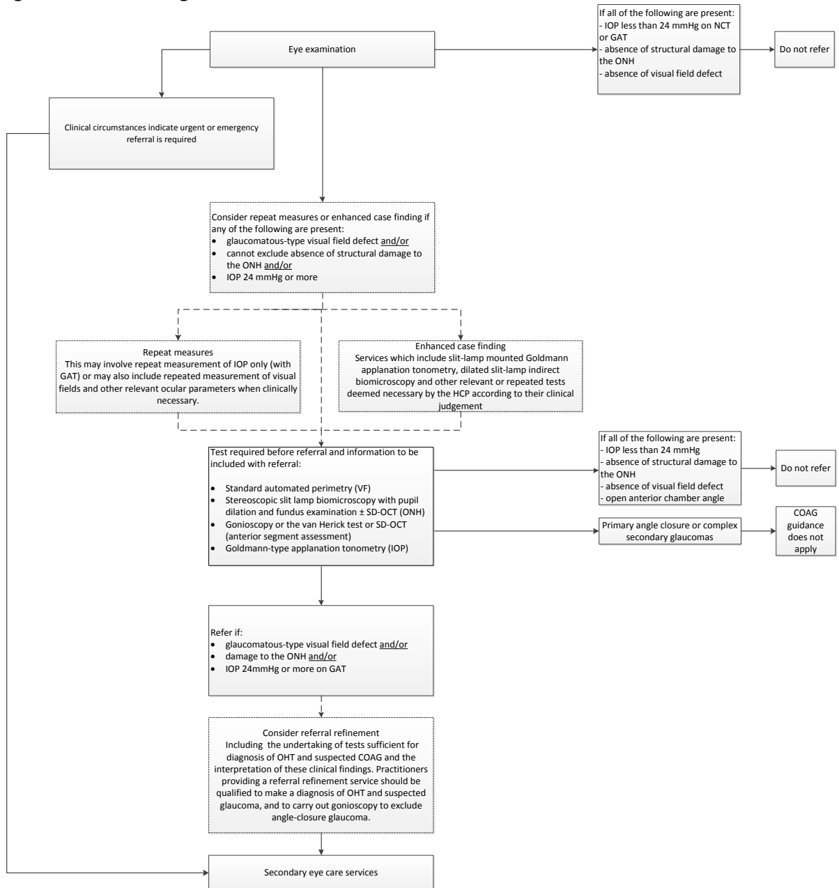
Figure 1: Referral algorithm
