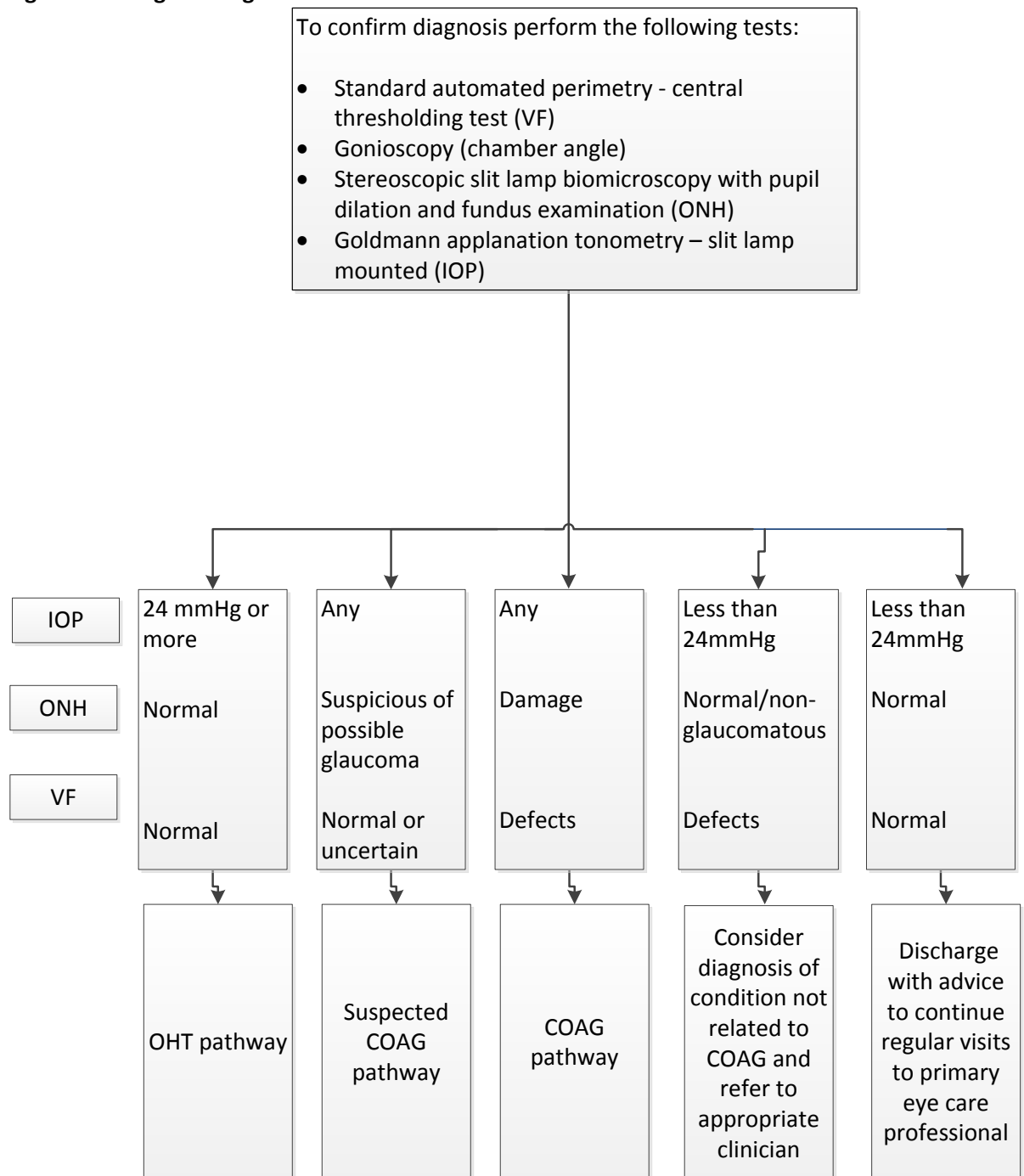
Figure 2: Diagnosis algorithm
