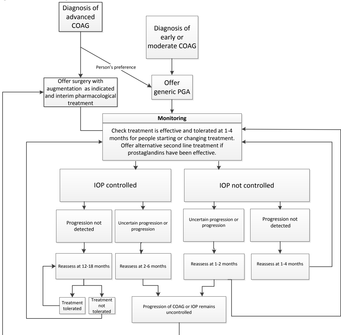
Figure 5: COAG algorithm
