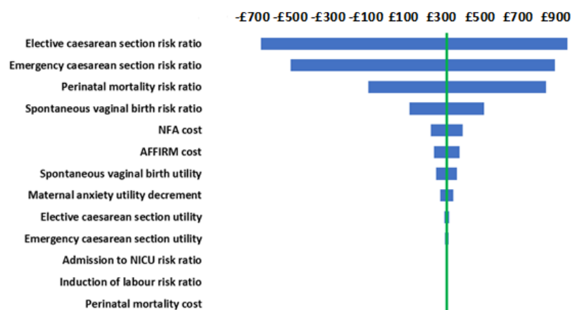
1 Figure 2: Tornado diagram displaying the effect of a high/low value of each parameter 2 on the incremental net monetary benefit, set at £20,000 per QALY: NFA 3 versus AFFIRM
