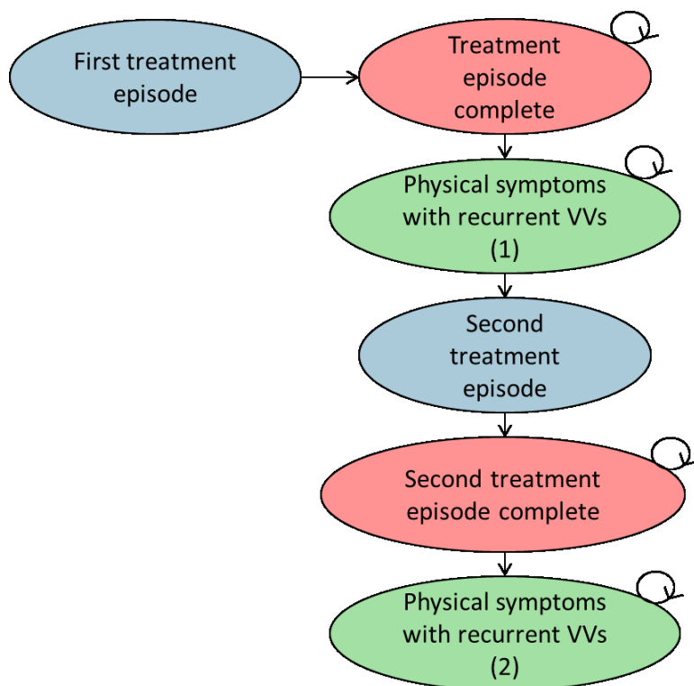
Figure 159: Model diagram
