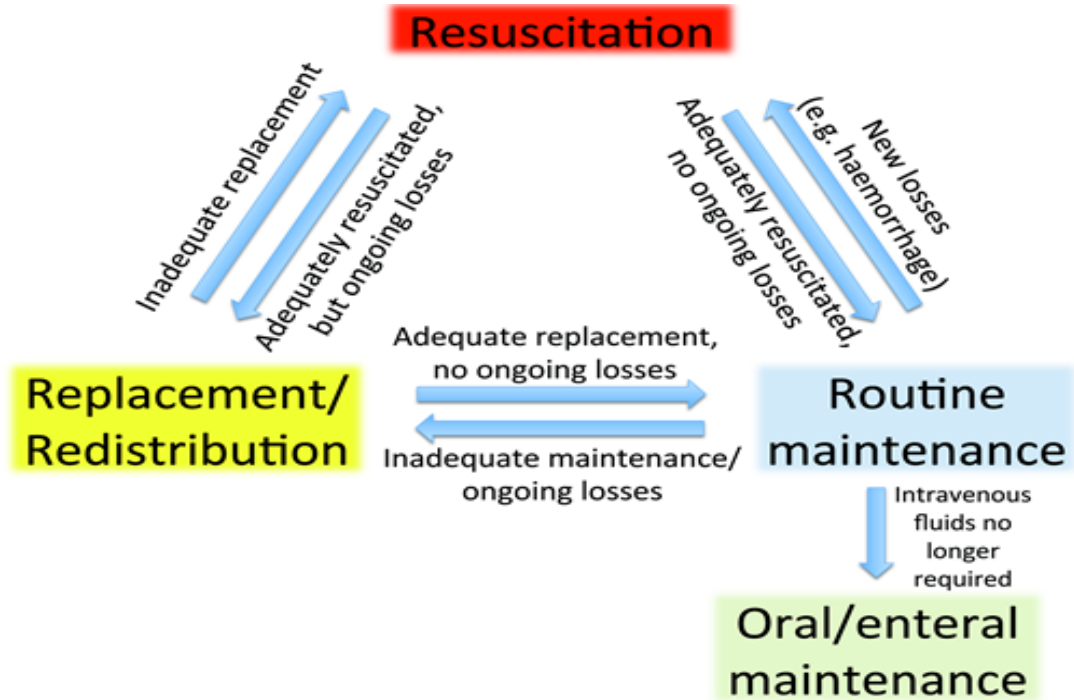
Figure 3: The 4 Rs - Resuscitation, Routine maintenance, Replacement and Redistribution. 58 A 5th R – Reassessment is also a critical element of care.
