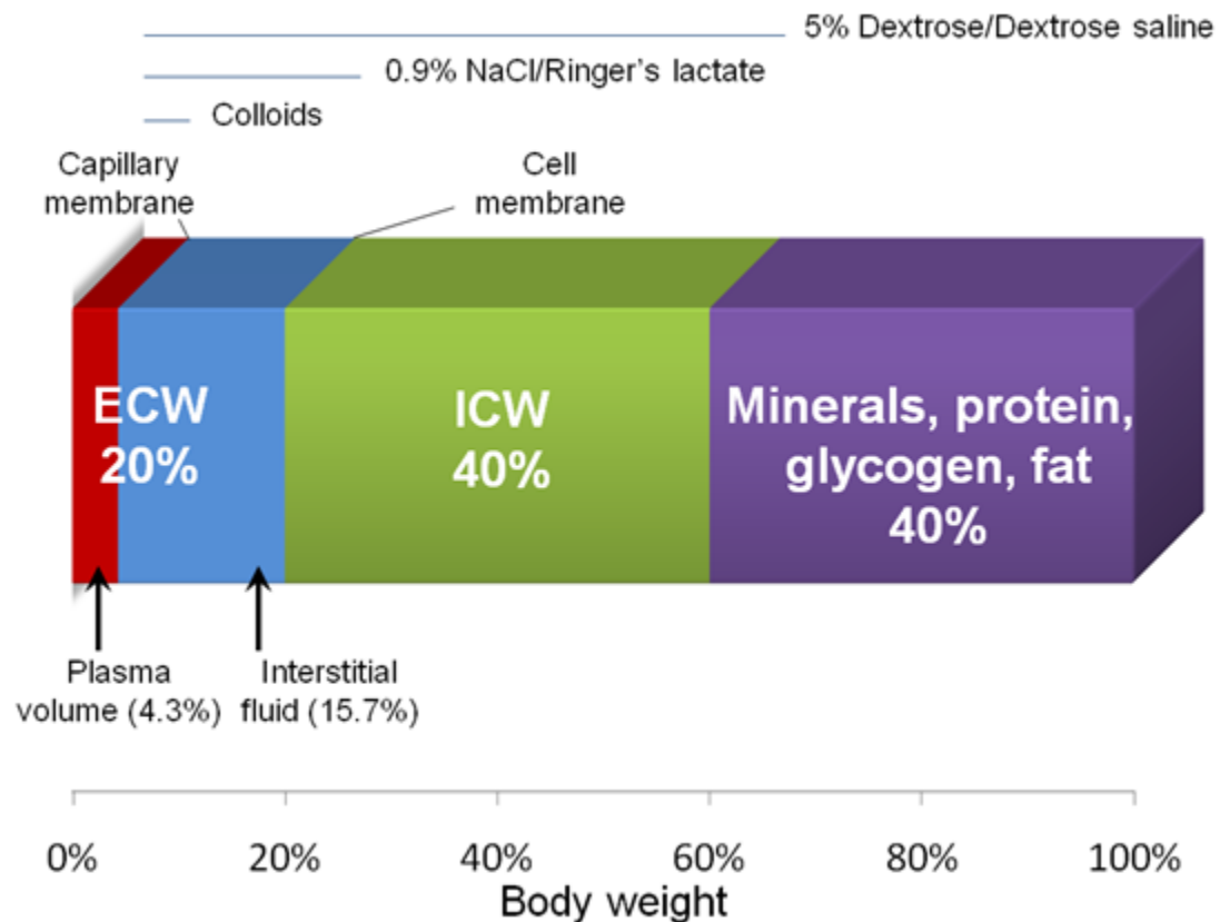
Figure 2: Body water compartments and approximate distribution of commonly used IV fluids
