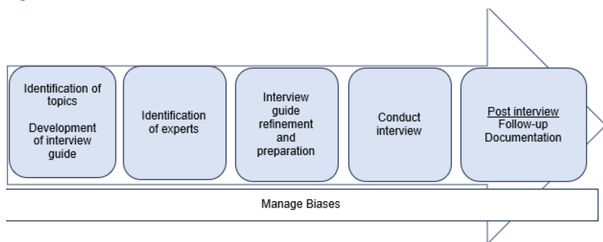
Figure 8. Elicitation Process
