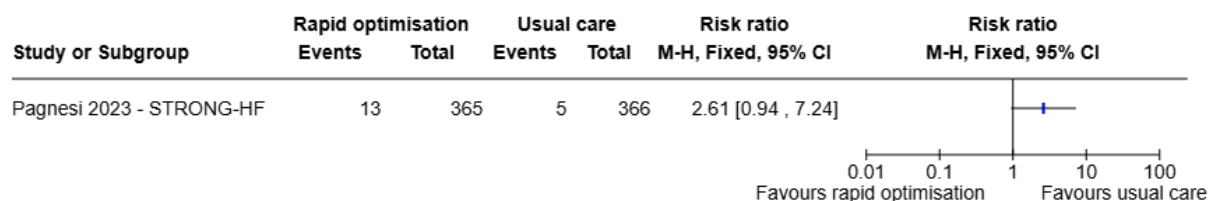
Figure 7: Hyperkalaemia (dichotomous)
