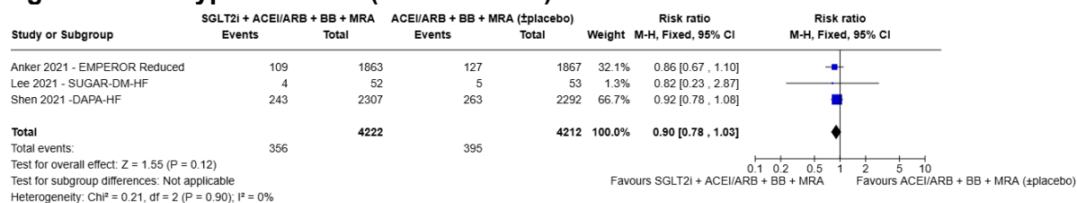
Figure 21: Hyperkalaemia (dichotomous)
