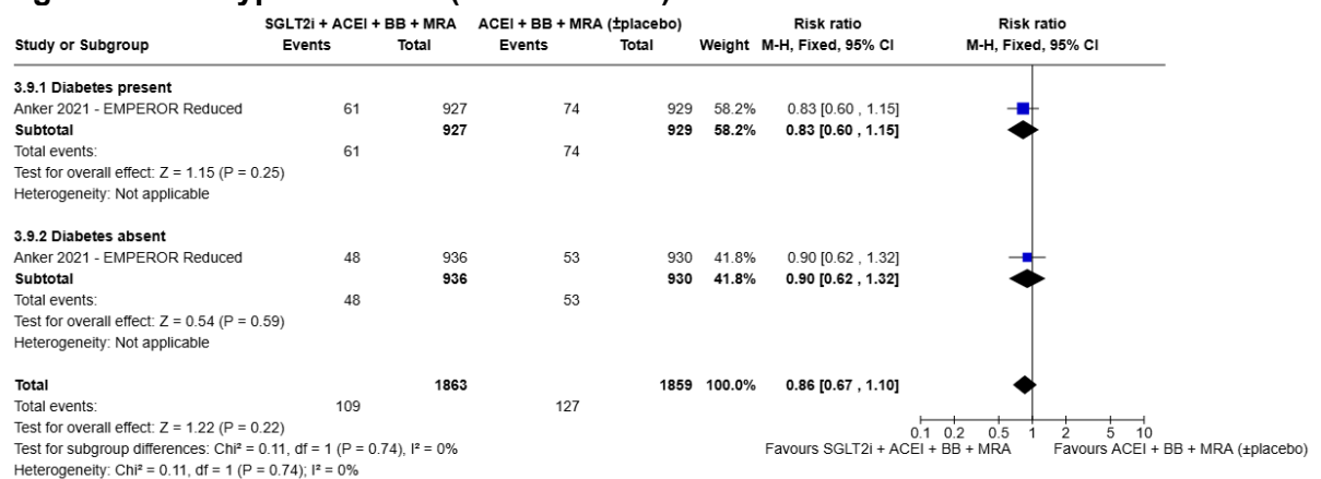
Figure 82: Hyperkalaemia (dichotomous)
