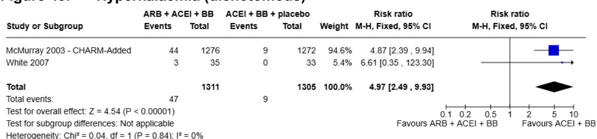
Figure 43: Hyperkalaemia (dichotomous)
