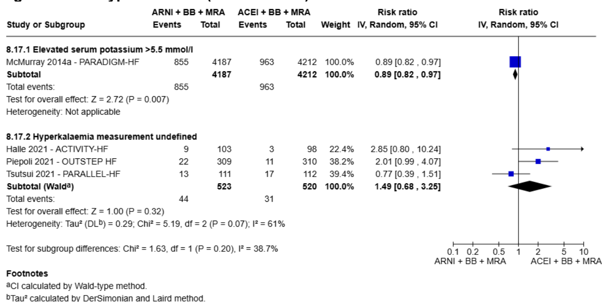
Figure 69: Hyperkalaemia (dichotomous)
