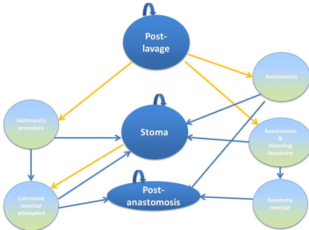
Figure 2: Markov model structure
