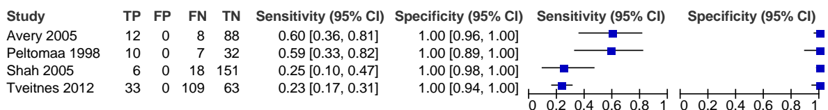
Figure 11: Sensitivity and specificity of Erythema migrans for diagnosing Lyme disease in children
