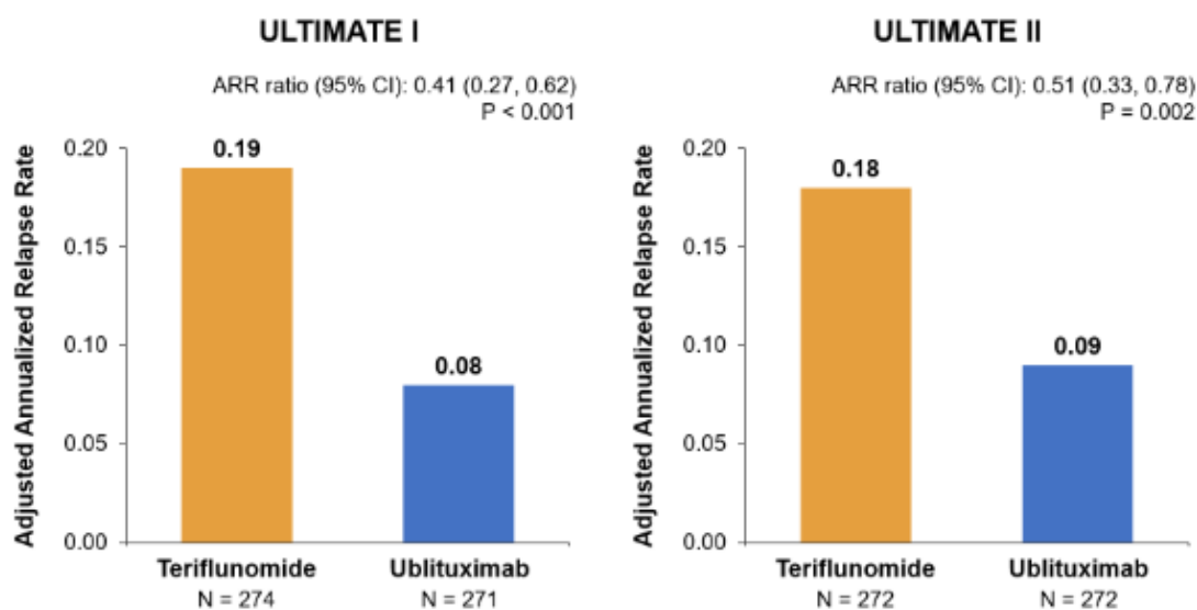
Figure 8 ARR over 96 weeks results in ULTIMATE I and II
