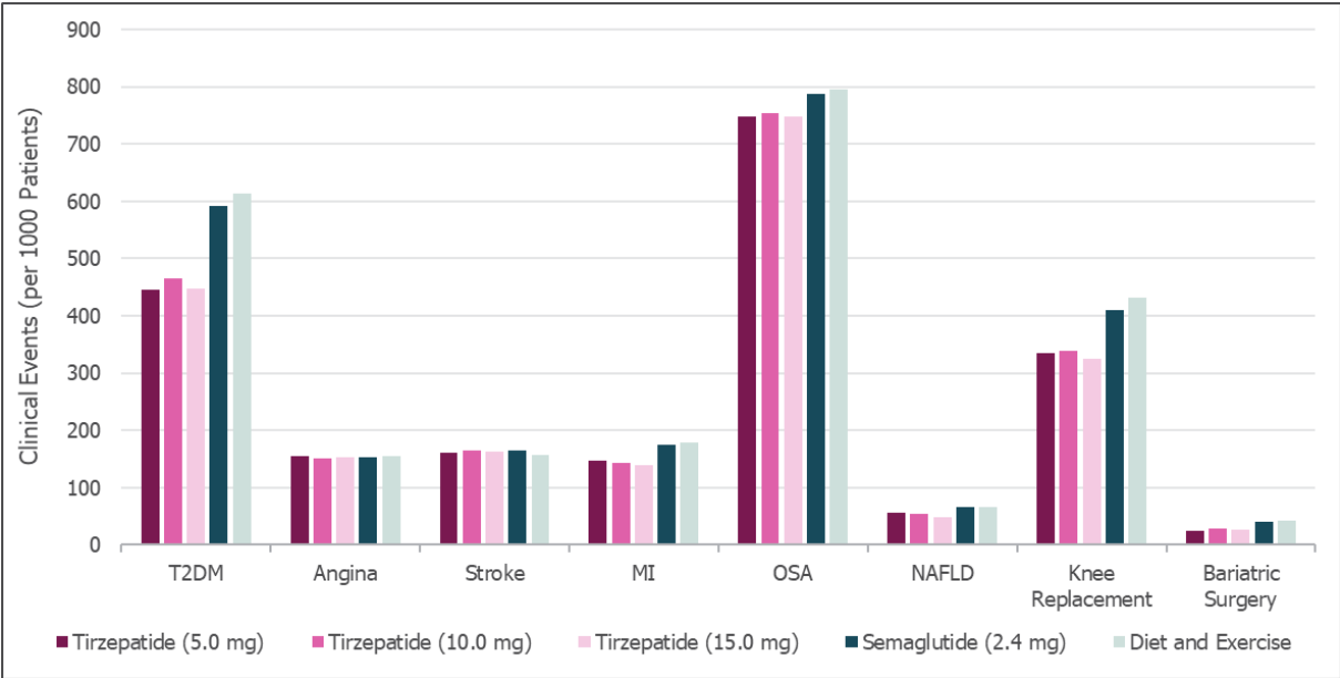
Figure 63: Base-case results for total incidences of clinical events over the model time horizon (deterministic)
