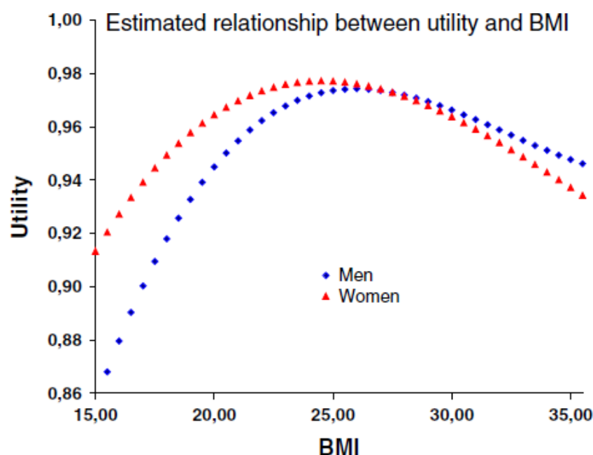
Figure 46: Relationship between EQ-5D and BMI, as reported in Søltoft et al. 2009 125
