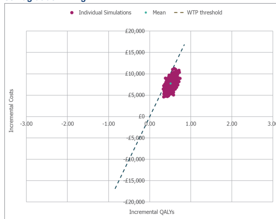
Figure 53: Cost-effectiveness plane for tirzepatide 10 mg versus semaglutide 2.4 mg
