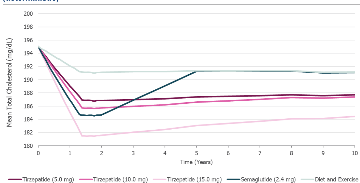
Figure 62: Base-case results for mean total cholesterol over first ten years of model (deterministic)
