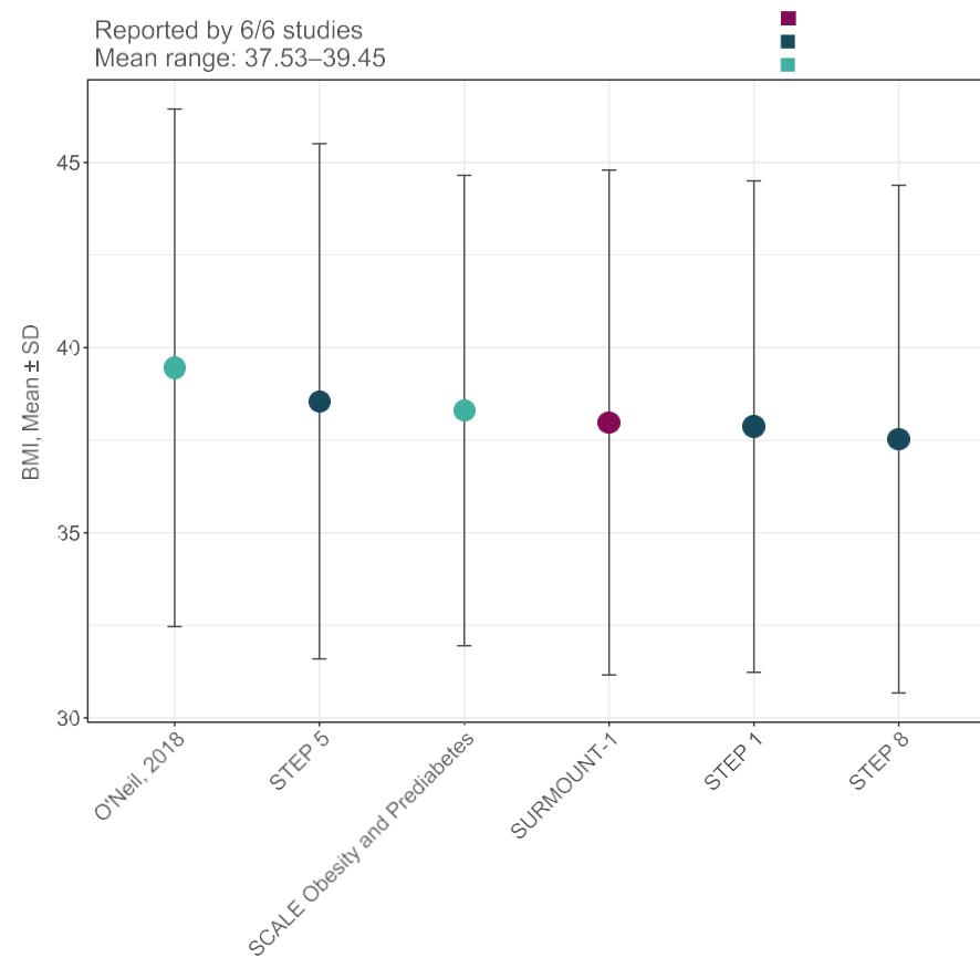
Figure 20. Heterogeneity assessment: BMI at baseline
