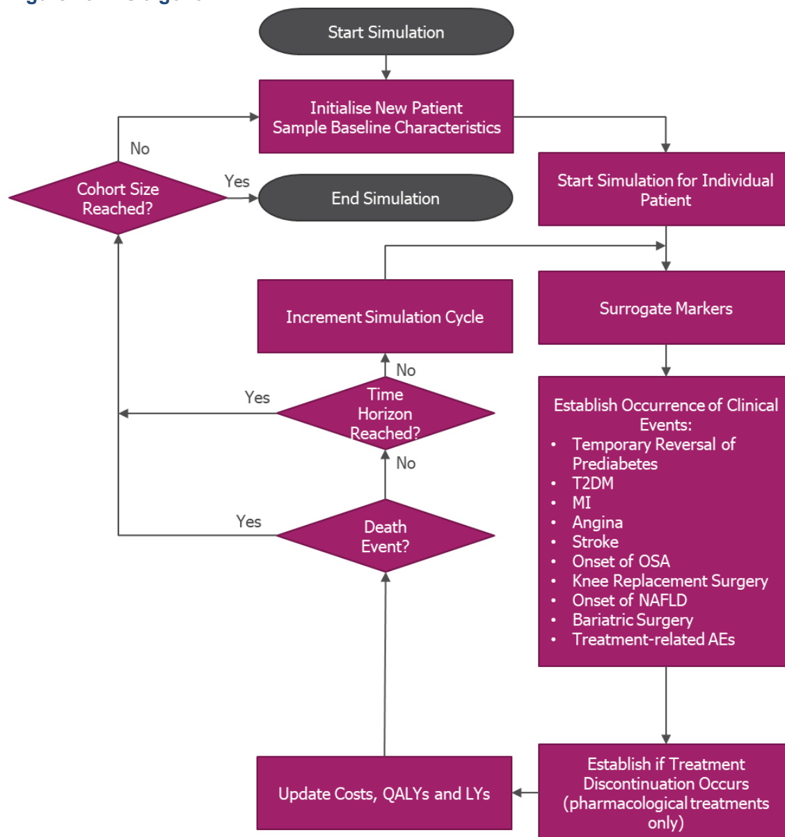
Figure 43: IPS algorithm
