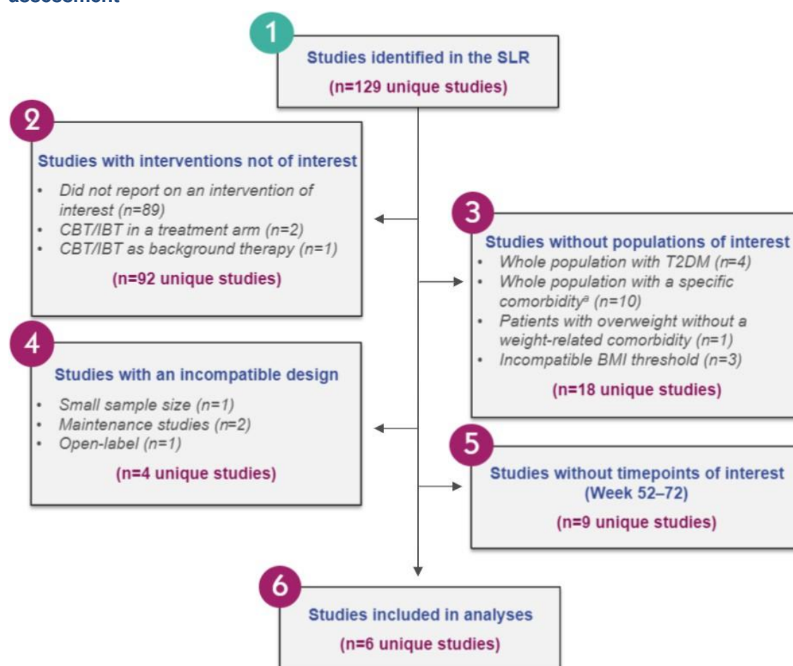
Figure 13. PRISMA diagram for study inclusion as assessed during the feasibility assessment
