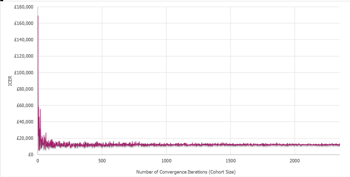
Figure 57: Cohort convergence plot for tirzepatide 10 mg versus diet and exercise
