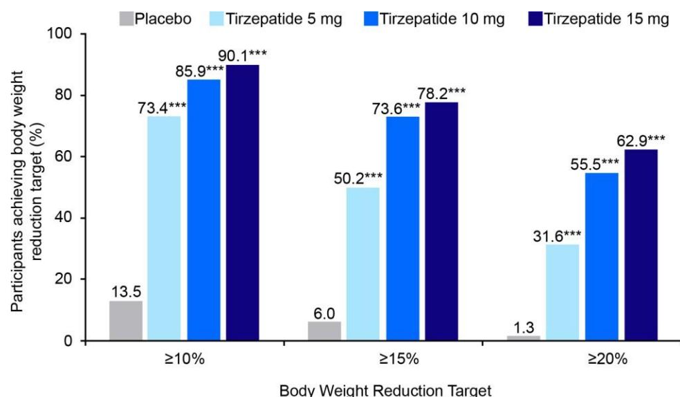
Figure 9. Percentage of participants achieving body weight reduction of \geq 10\% , \geq 15\% , or \geq 20\% at Week 72; EAS
