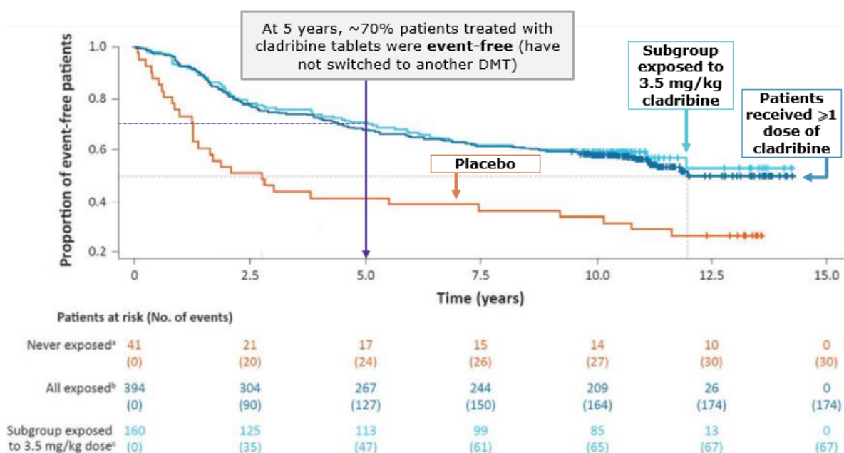
Figure 9: Kaplan–Meier curve for time to first subsequent DMT after last parent study dose in CLARITY/CLARITY-EXT (CLASSIC-MS)
