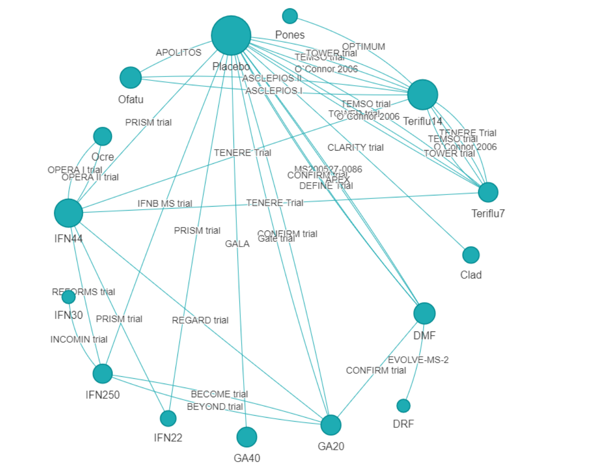
Figure 16: Network diagram for the base case NMA of treatment discontinuation (ITT population)
