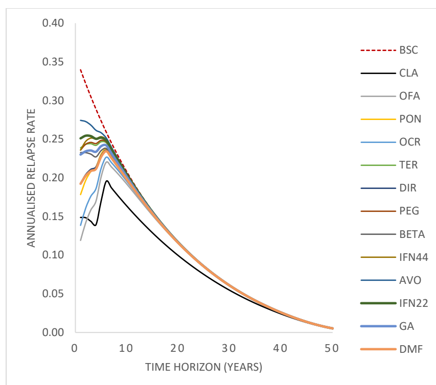
Figure 20. Predicted number of relapses over the modelled time horizon
