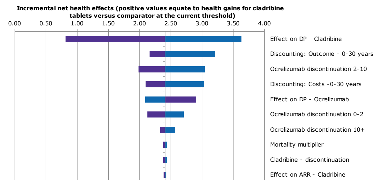
Figure 24: Tornado diagram for active RRMS, cladribine tablets versus ocrelizumab
