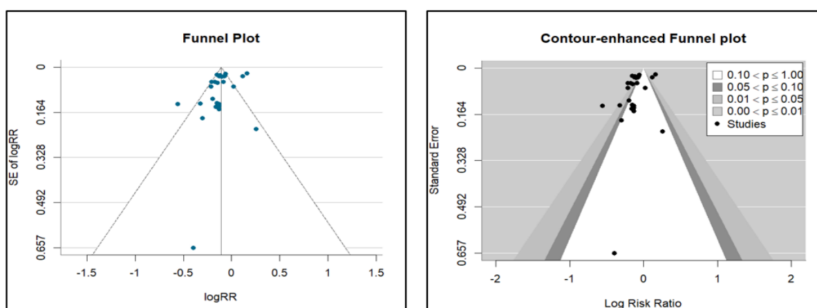
Figure 2. Funnel plot and contour-enhanced funnel plot for studies reporting ARR (Figure 3 from the CS, Appendix D.1.1.5).
