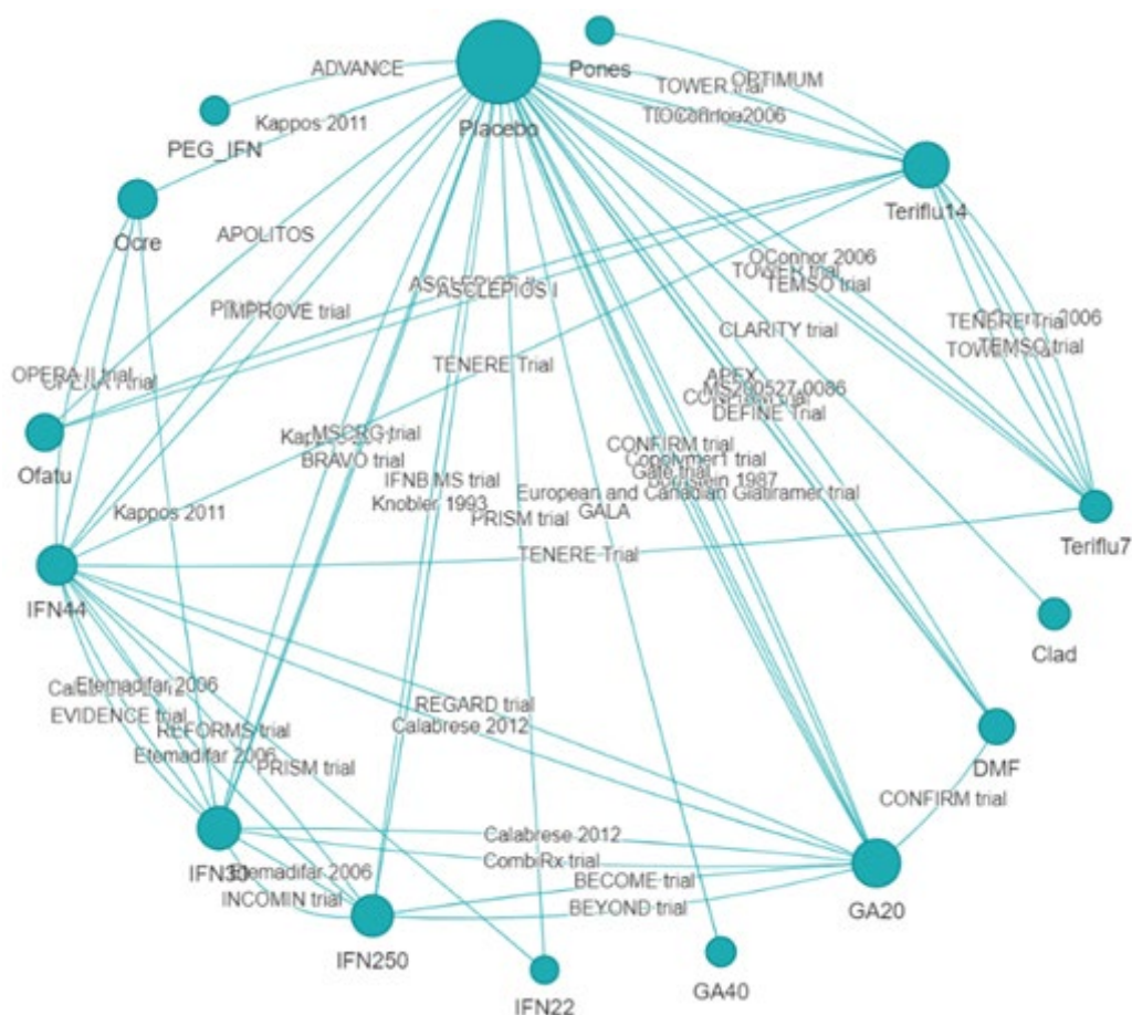
Figure 10: Network diagram for the base case NMA of ARR
