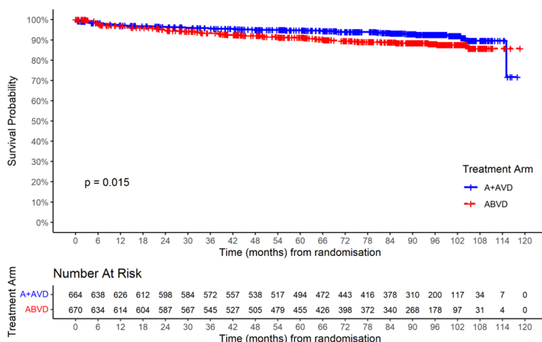
Figure 12: OS Kaplan–Meier | ITT population | March 2023 DCO
