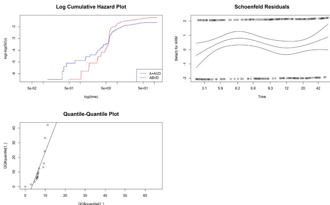
Figure 19: PFS proportional hazards and accelerated failure time tests
