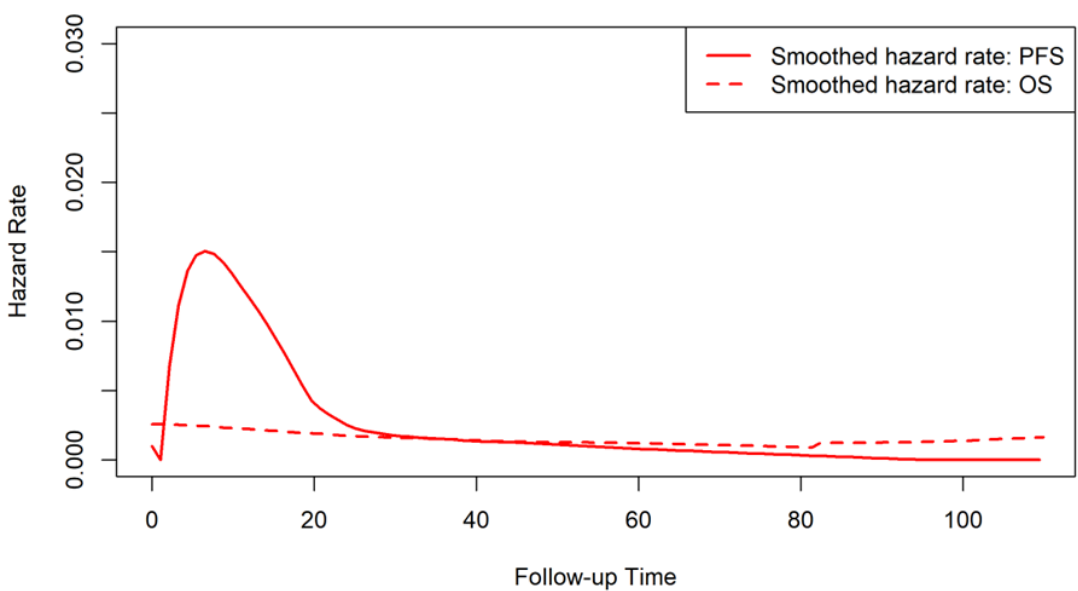
Figure 9. ABVD (ITT population) smoothed hazard plots (reproduced from Figure 25 in the CQ response)
