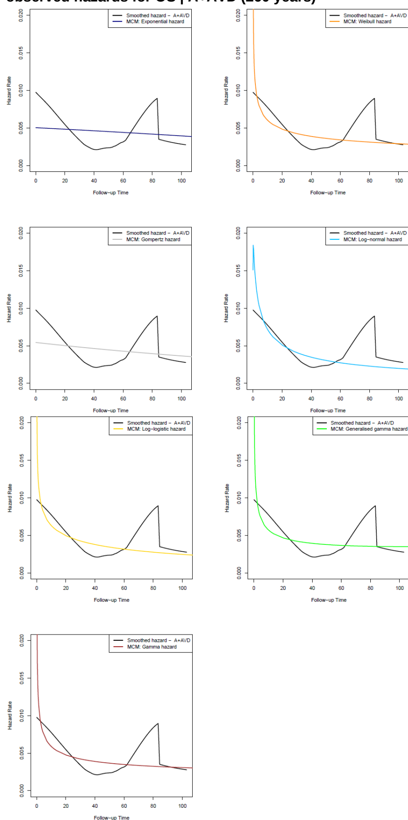
Figure 96: Comparison of predicted independent MCM parametric models and observed hazards for OS | A+AVD ( \geq 60 years)
