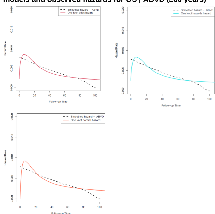
Figure 102: Comparison of predicted independent one-knot splines parametric models and observed hazards for OS | ABVD (≥60 years)
