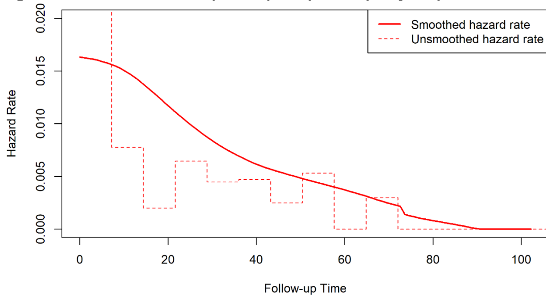
Figure 75: Observed hazards | ABVD | PFS per INV ( \geq 60 years)
