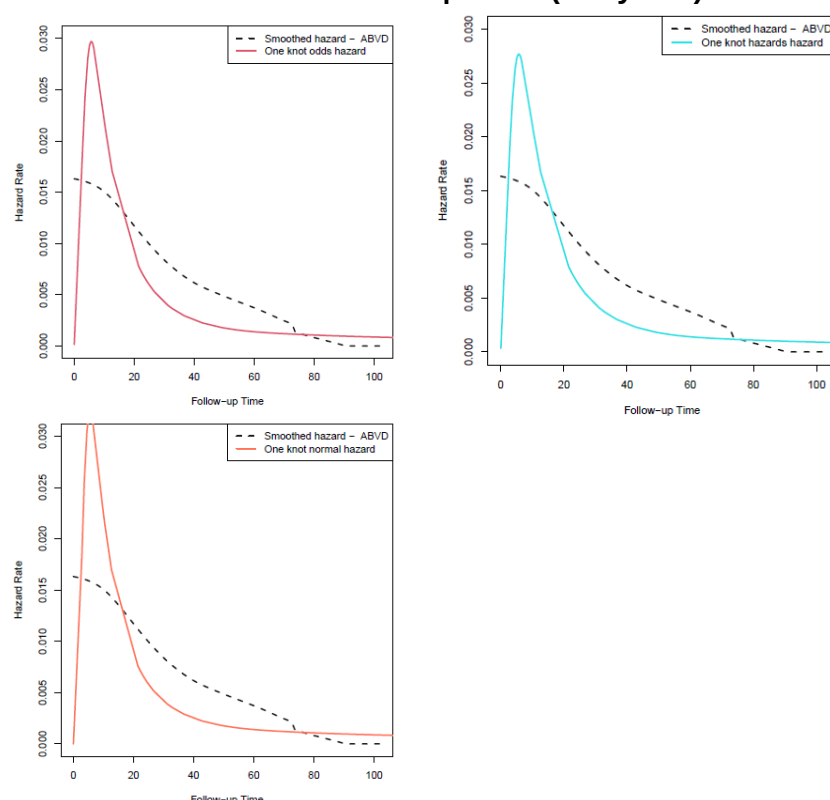
Figure 87: Comparison of predicted independent one-knot splines parametric models and observed hazards for PFS | ABVD ( \geq 60 years)
