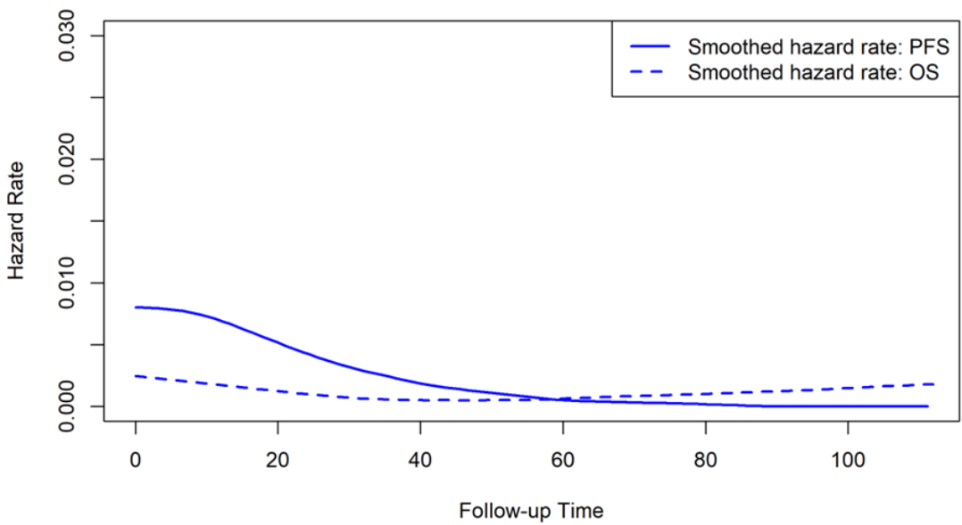
Figure 8. A+AVD (ITT population) smoothed hazard curves (reproduced from Figure 24 in the CQ response)
