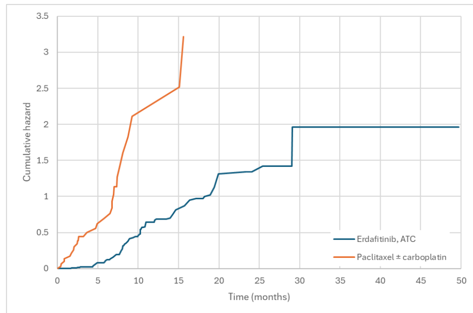
Figure 15. Cumulative hazard over time for OS of ATC-adjusted erdafitinib versus paclitaxel ± carboplatin, missing data excluded
