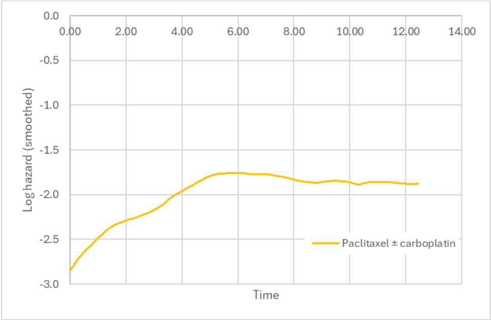
Figure 23. Log smoothed hazard over time – OS, paclitaxel ± carboplatin
