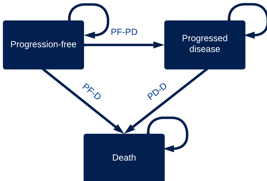
Figure 31. Three-state semi-Markov model structure
