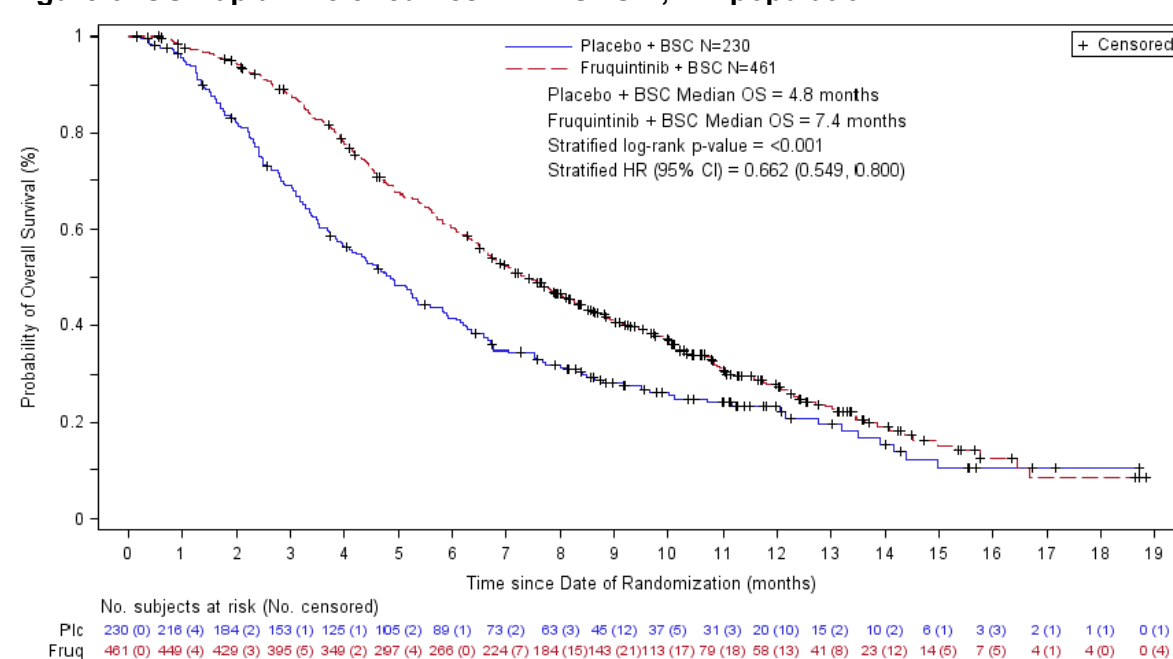
Figure 6: OS Kaplan-Meier curves – FRESCO-2, ITT population
