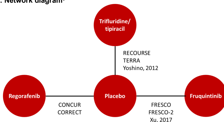
Figure 17: Network diagram †
