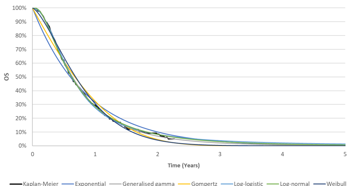
Figure 10: Parametric fits for OS compared with KM data, trifluridine-tipiracil (Pooled RECURSE and Yoshino et al)
