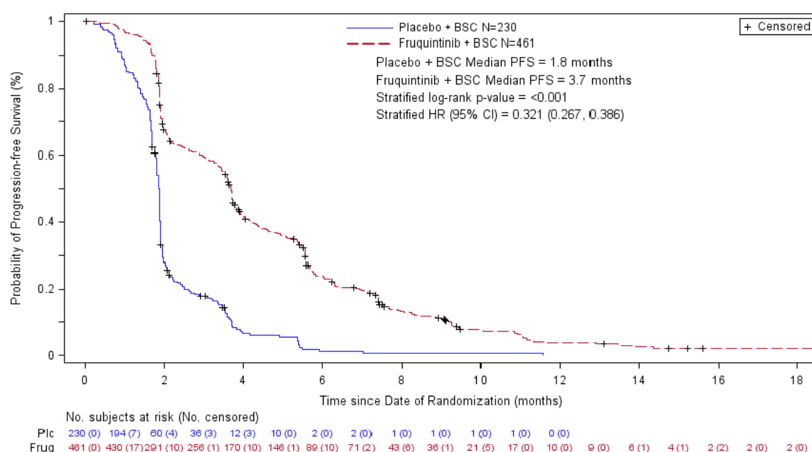
Figure 8: PFS Kaplan-Meier curves – FRESCO-2, ITT population
