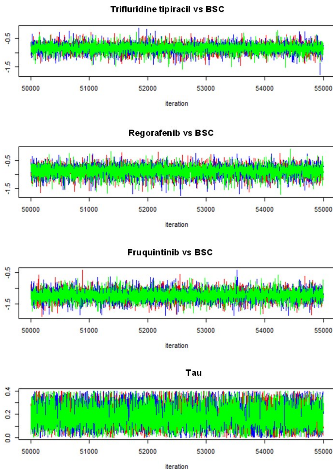
Figure 29: Base case: PFS random effects – trace plot
