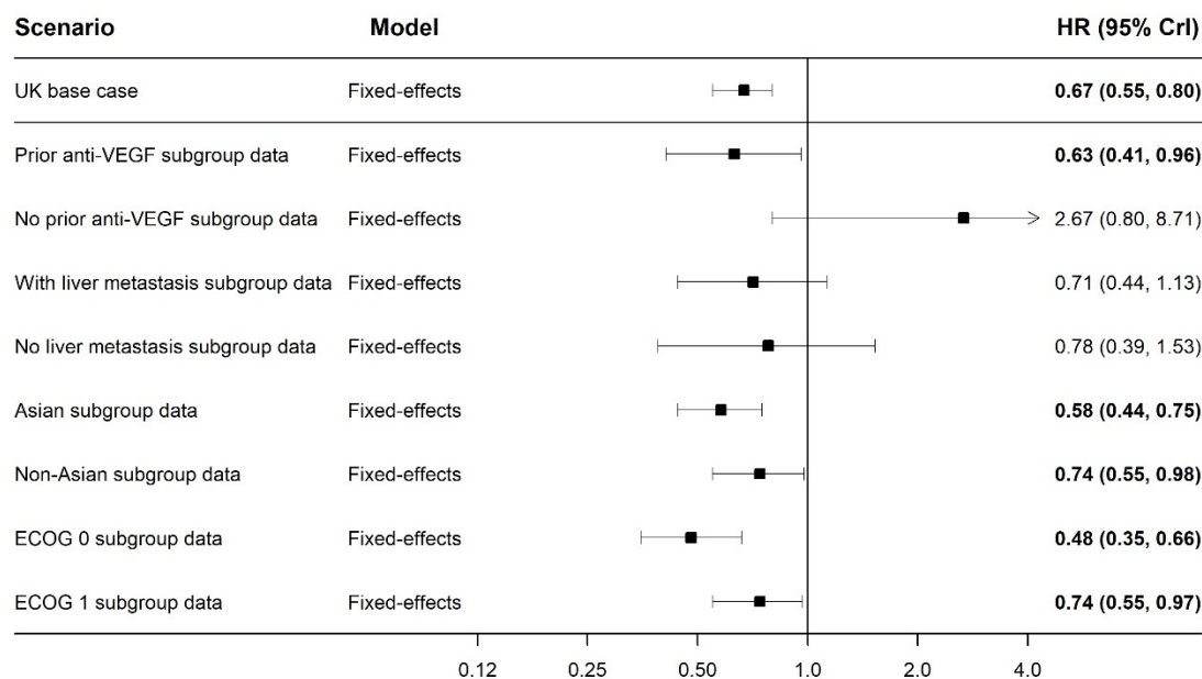
Figure 27: Forest plot PFS fruquintinib vs trifluridine-tipiracil (fixed effects scenario analyses)
