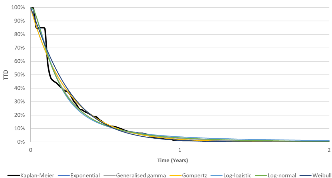
Figure 12: Parametric fits for TTD compared with KM data, trifluridine-tipiracil
