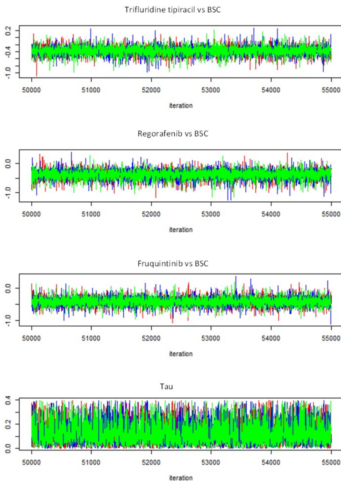
Figure 25: Base case: OS random effects – trace plot
