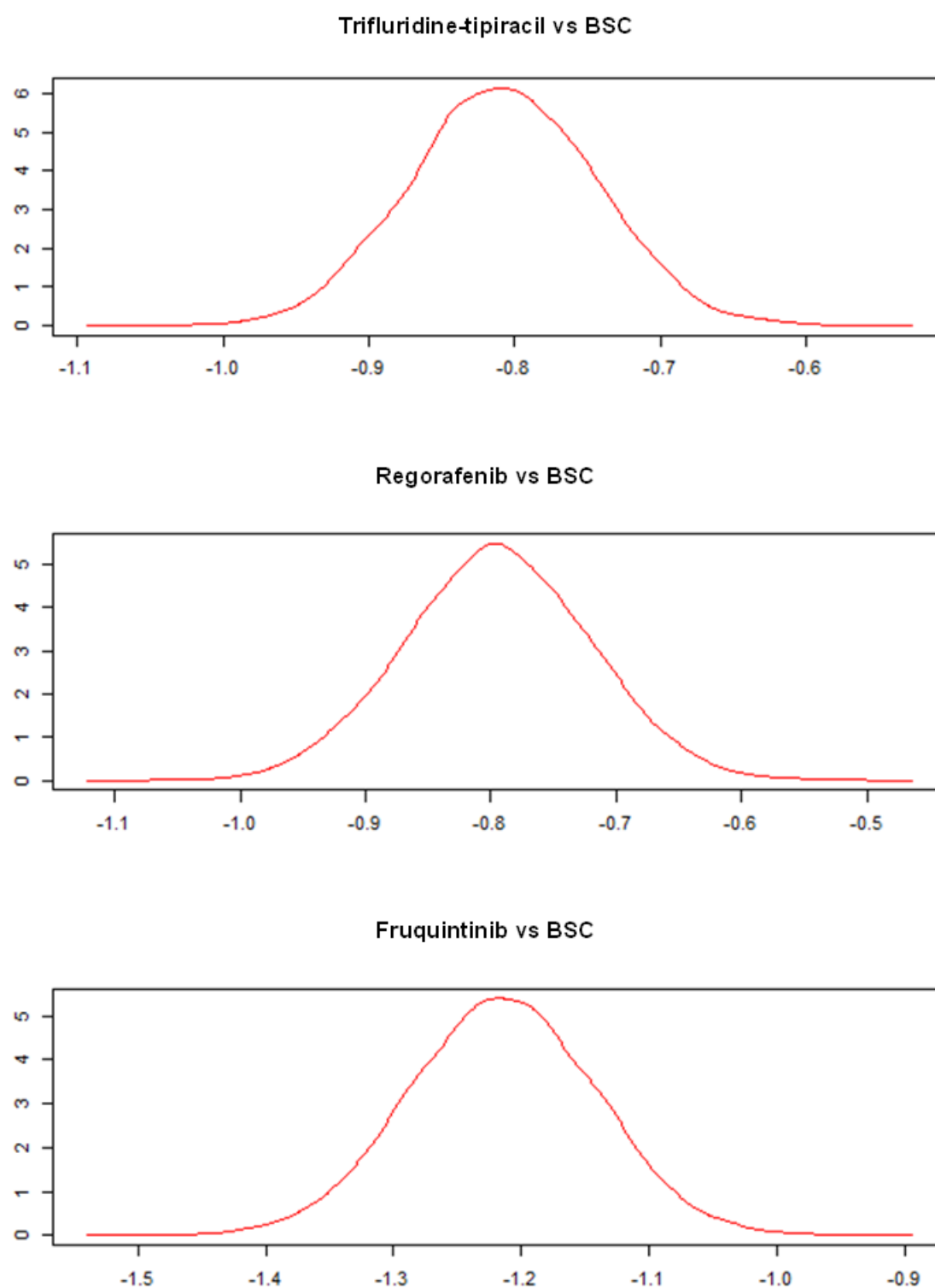
Figure 28: Base case: PFS fixed effects – density plot
