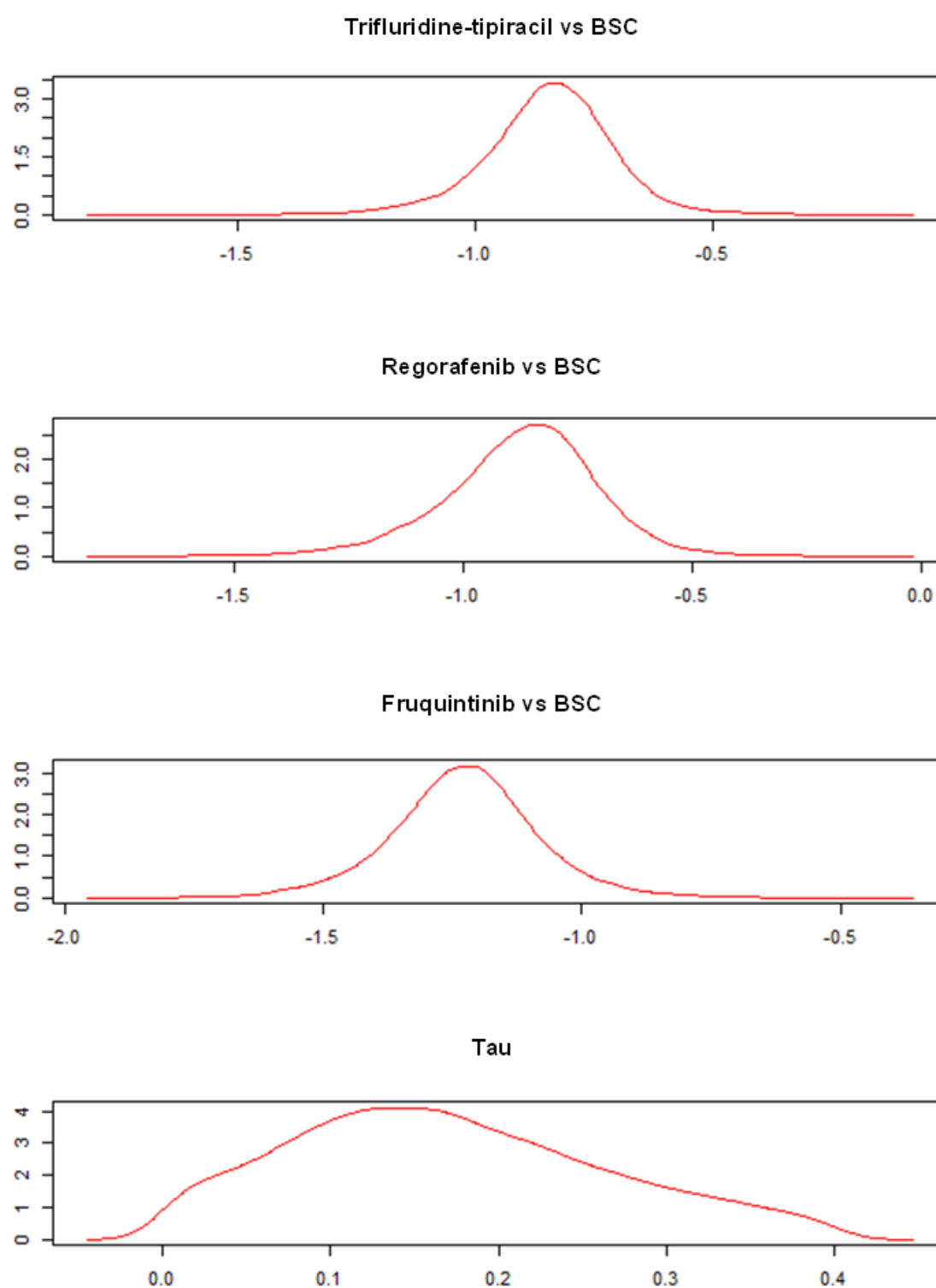
Figure 30: Base case: PFS random effects – density plot
