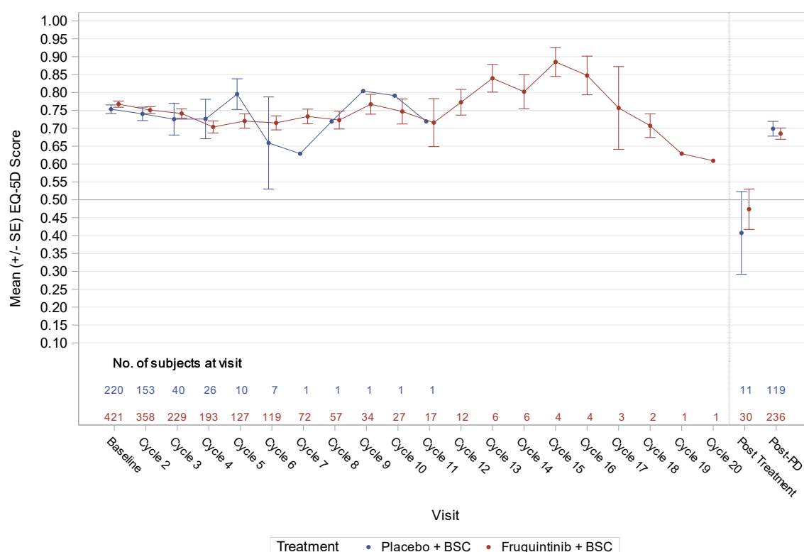
Figure 22: Mean EQ-5D-3L score by visit
