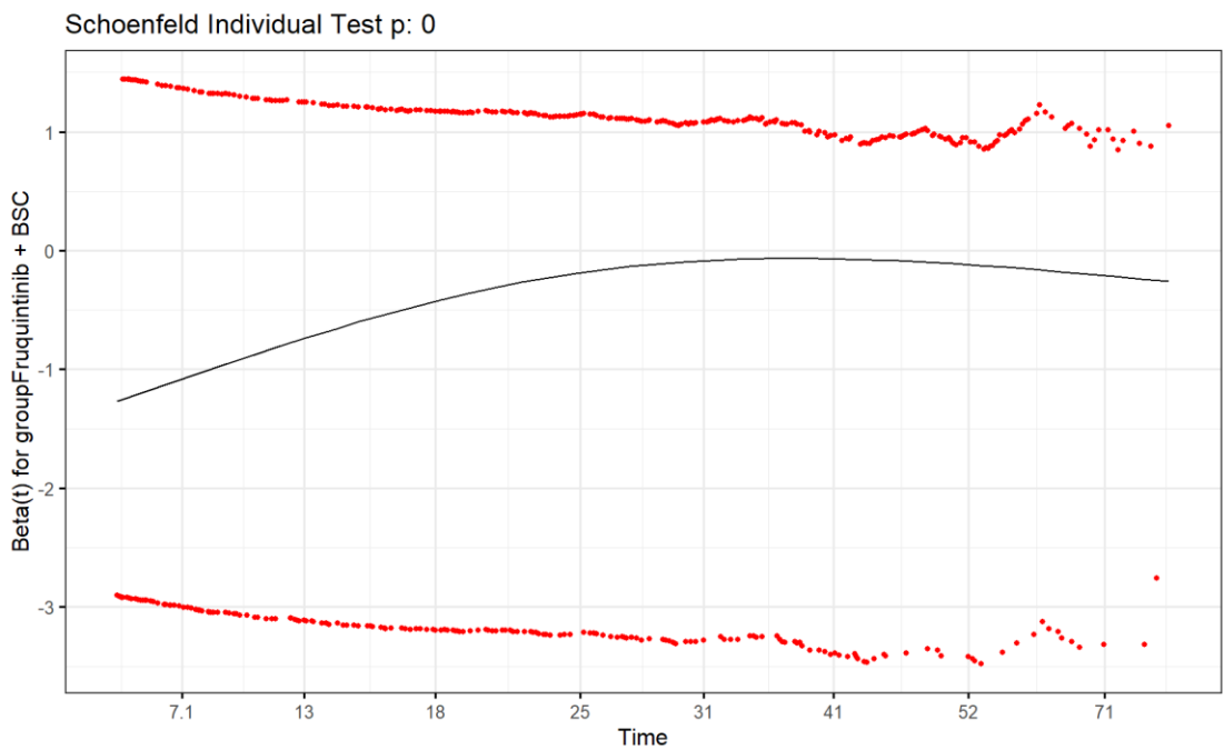
Figure 31: Schoenfeld residual plot, pooled data, OS
