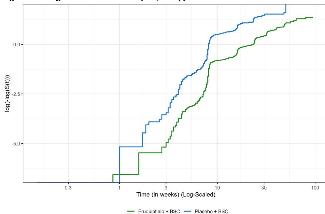
Figure 37: Log cumulative hazard plot, PFS, pooled data
