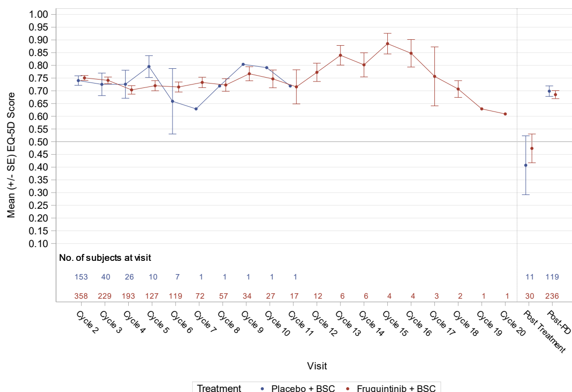
Figure 46: Mean EQ-5D-3L score by visit
