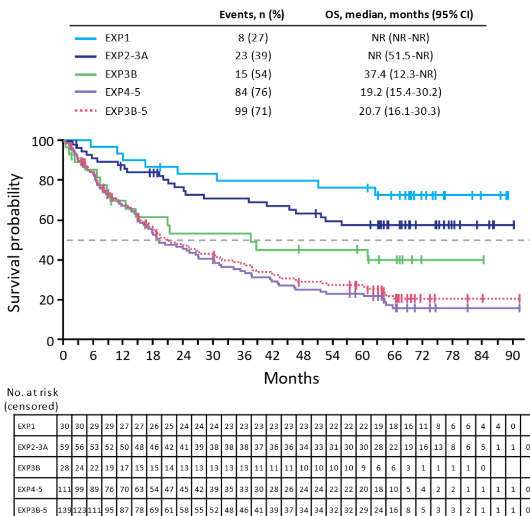
Figure 12 Kaplan-Meier OS curve in ALK-positive patients: cohorts of Study 1001
