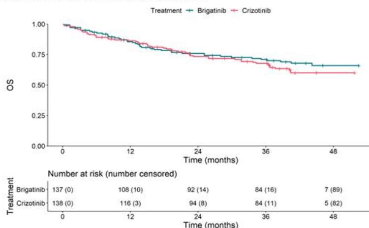
Kaplan-Meier curve for OS in ALTA-1
