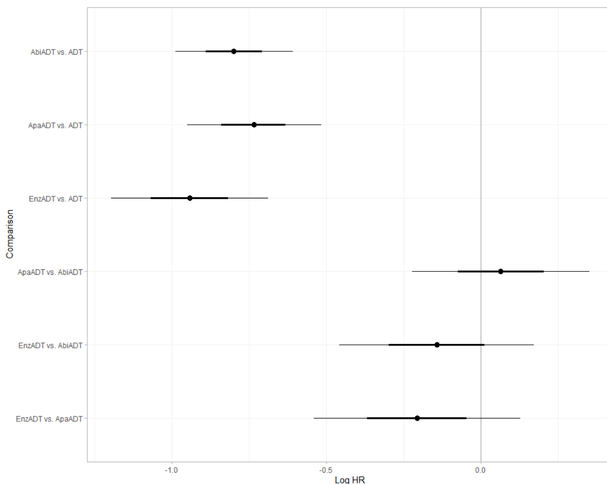
Figure 26: Forest plot of rPFS sensitivity analysis results in terms of the logarithm of HR:
