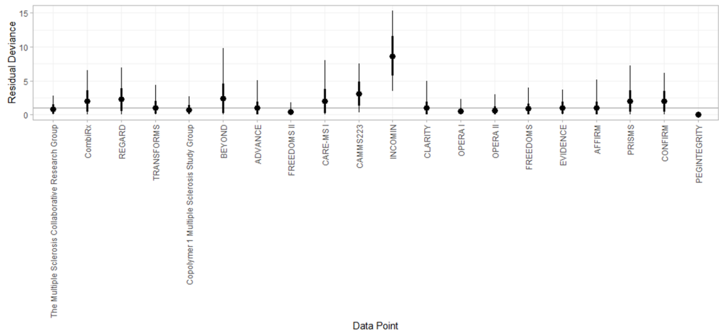
Figure 35 Model fit for CDP3 and CDP6 combined assessed by individual study residual deviance (random effects analysis; RRMS population)
