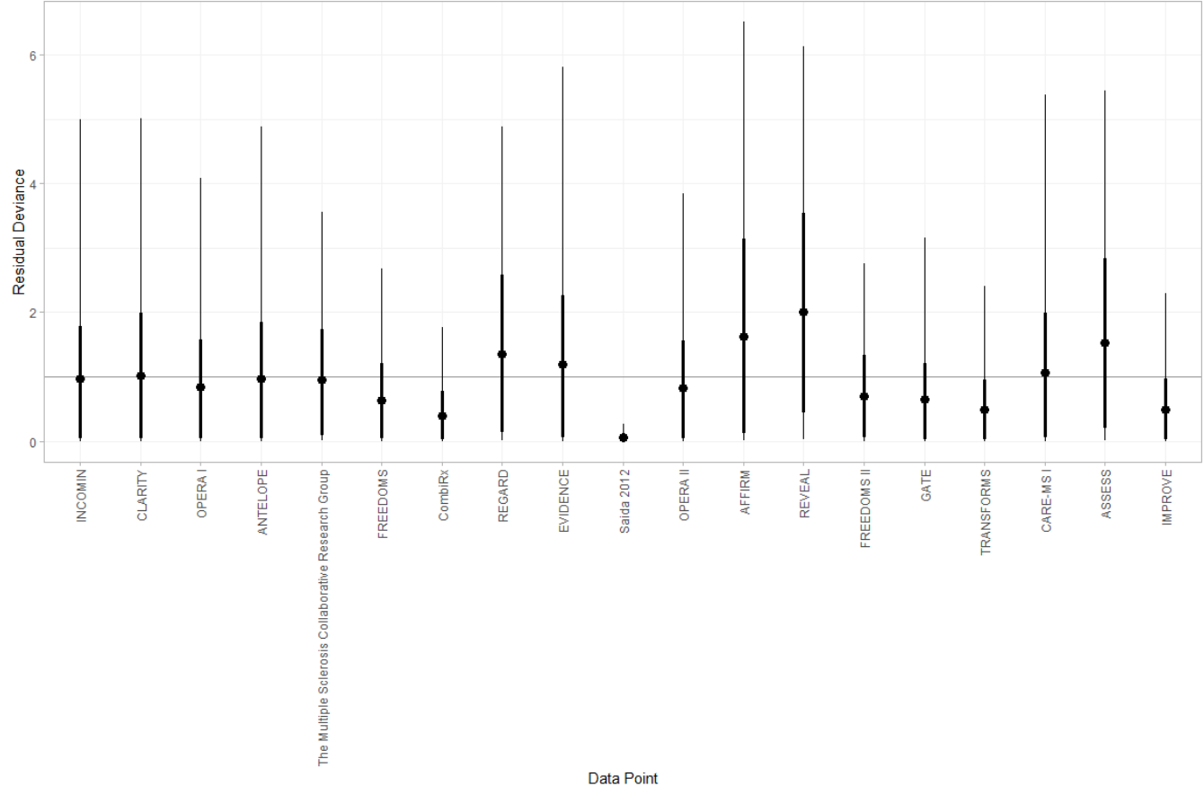
Figure 36 Model fit for MRI Gd+ lesions combined assessed by individual study residual deviance (fixed effects analysis; RRMS population)
