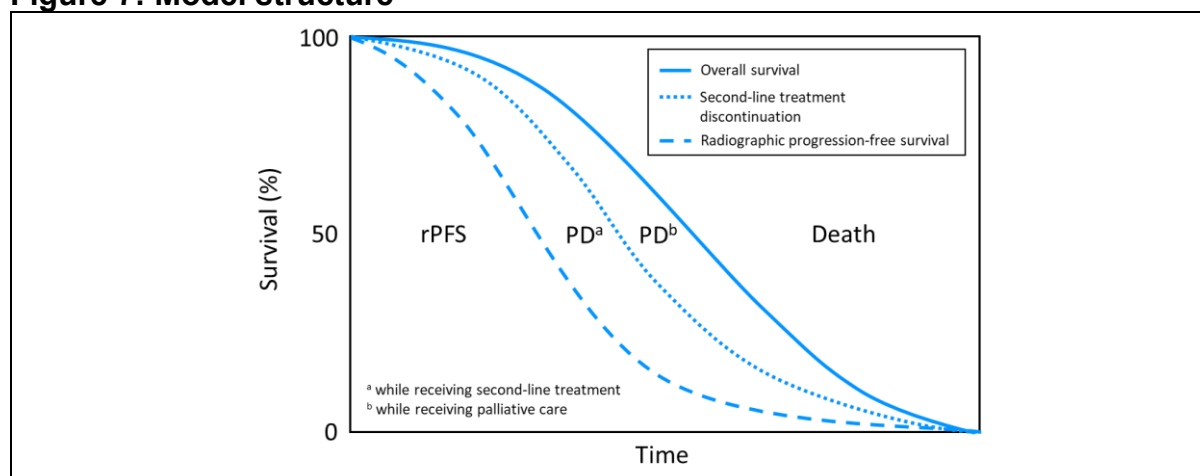
Figure 7: Model structure
