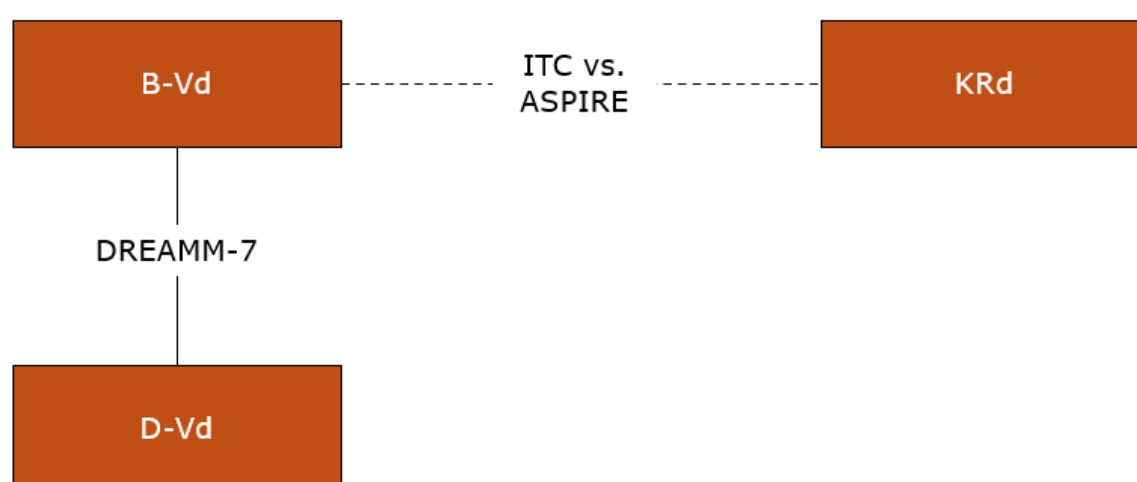
Figure 1. Indirect network of evidence
