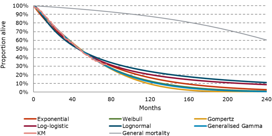
Figure 21: OS independent curves for unweighted KRd
