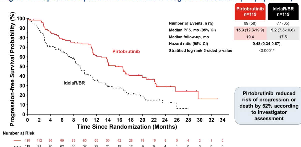
Figure 10: Kaplan Meier plot of PFS based on Investigator Assessment (ITT population)
