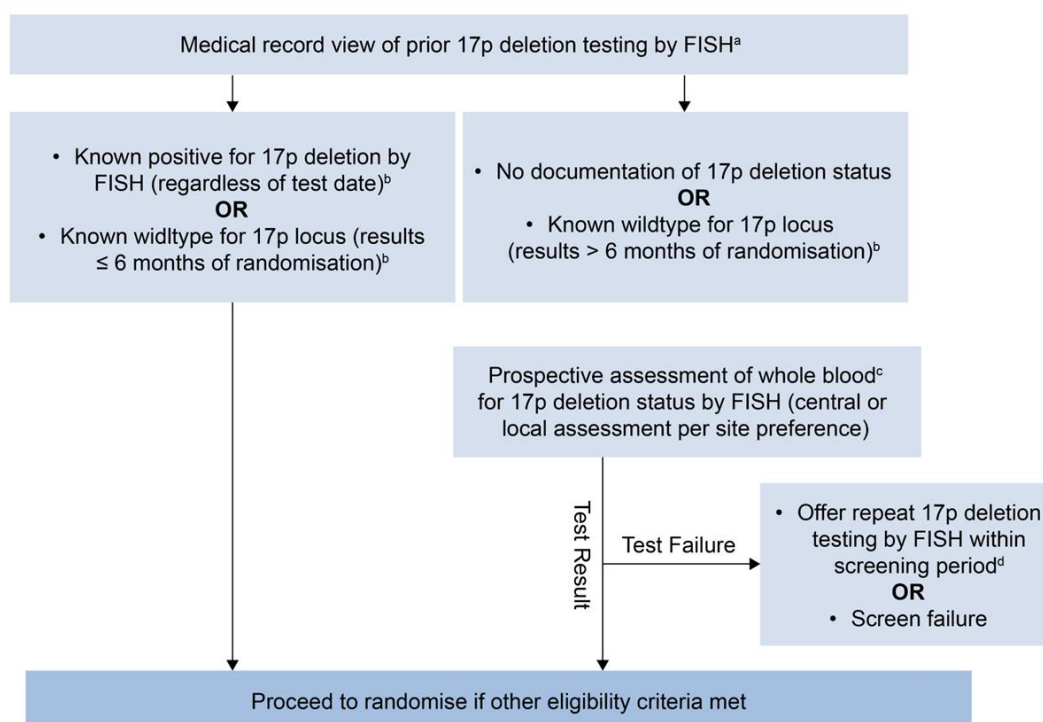
Figure 4: Schema for 17p deletion stratification
