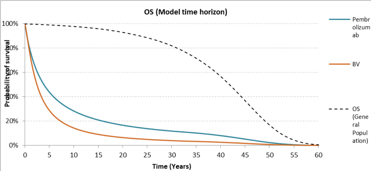
Figure 8: Comparison of OS; SACT data and Eyre preferred extrapolations
