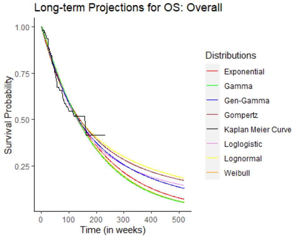
Figure 5: Long term OS projections for BV in Eyre (2017)
