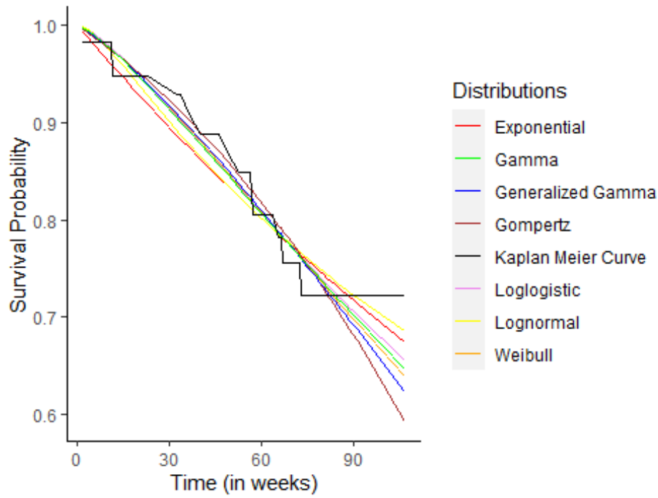
Parametric Fitting for OS: ITT
