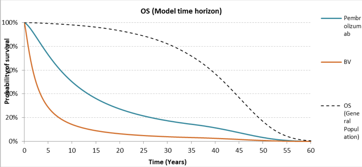
Figure 7: Comparison of OS; KN-087 and Eyre - preferred extrapolations
